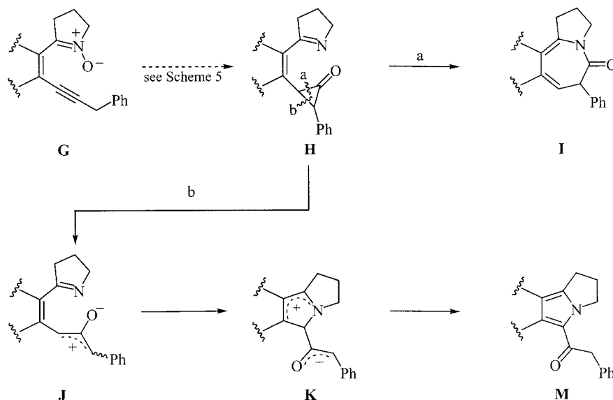
Scheme 14. Reagents and conditions: (i) \text{BrMg}(\text{CH}_2)_4\text{Cl} , THF, -40^\circ\text{C} ; (ii) IBX, DMSO, room temp.; (iii) \text{NH}_2\text{OH}\cdot\text{HCl} , \text{K}_2\text{CO}_3 , EtOH/ \text{H}_2\text{O} , reflux; (iv) KOH, TBAI, toluene, reflux.
