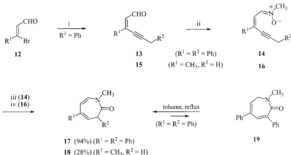
Scheme 4. Reagents and conditions: (i) and (ii) as for Scheme 3; (iii) MeONa, MeOH, 30 min, room temp.; (iv) NaH, DMF, 22 h, 60 °C.
