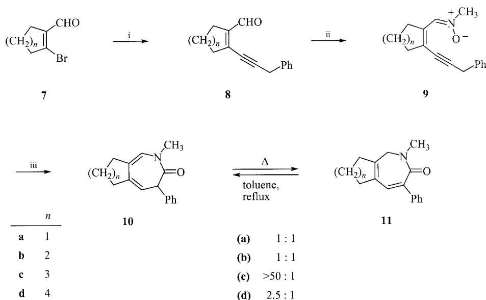
Scheme 3. Reagents and conditions: (i) HC≡CCH 2 Ph, PdCl 2 (PPh 3 ) 2 , CuI, NEt 3 , C 6 H 6 ; (ii) CH 3 NHOH·HCl, NaOAc, CH 2 Cl 2 ; (iii) KOH, MeOH, room temp.
