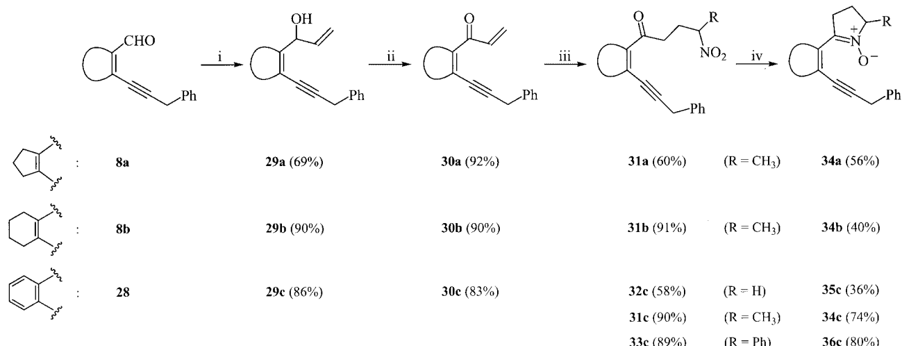
Scheme 9. Reagents and conditions: (i) vinylmagnesium bromide, THF; (ii) IBX, DMSO, room temp.; (iii) RCH 2 NO 2 , i Pr 2 NH, CHCl 3 ; (iv) Fe, HCl, EtOH, reflux.
