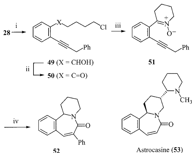
Scheme 14. Reagents and conditions: (i) \text{BrMg}(\text{CH}_2)_4\text{Cl} , THF, -40^\circ\text{C} ; (ii) IBX, DMSO, room temp.; (iii) \text{NH}_2\text{OH}\cdot\text{HCl} , \text{K}_2\text{CO}_3 , EtOH/ \text{H}_2\text{O} , reflux; (iv) KOH, TBAI, toluene, reflux.
